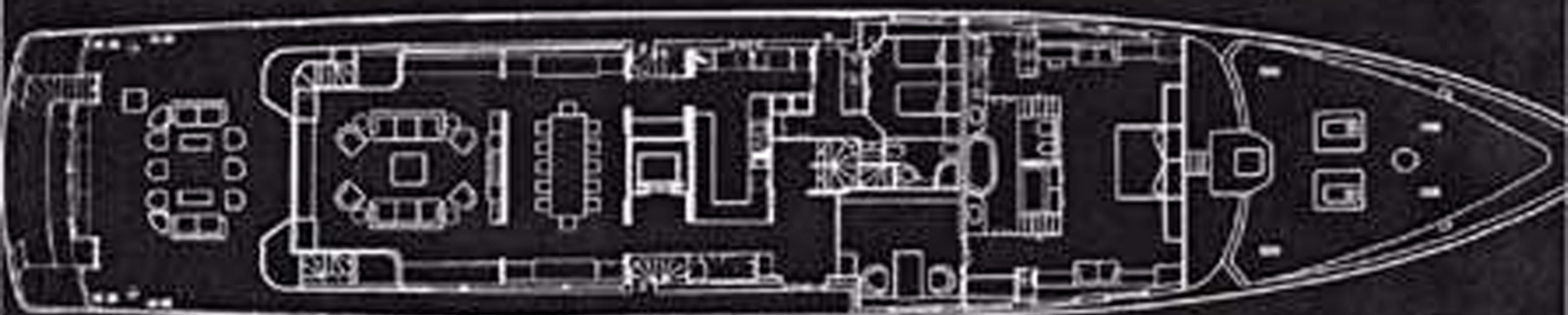
MAIN DECK
